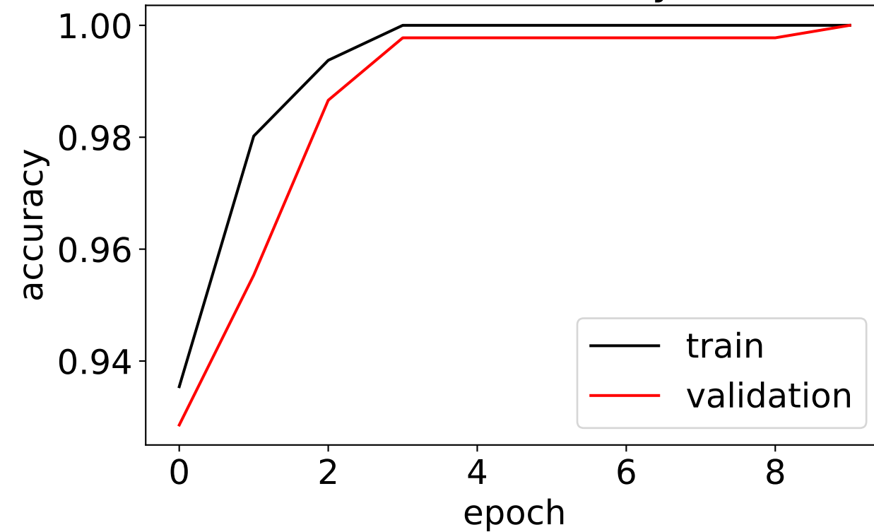
C model accuracy
