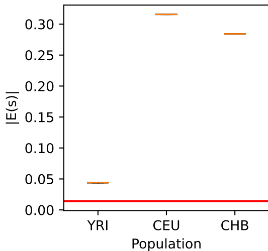
polyDFE
