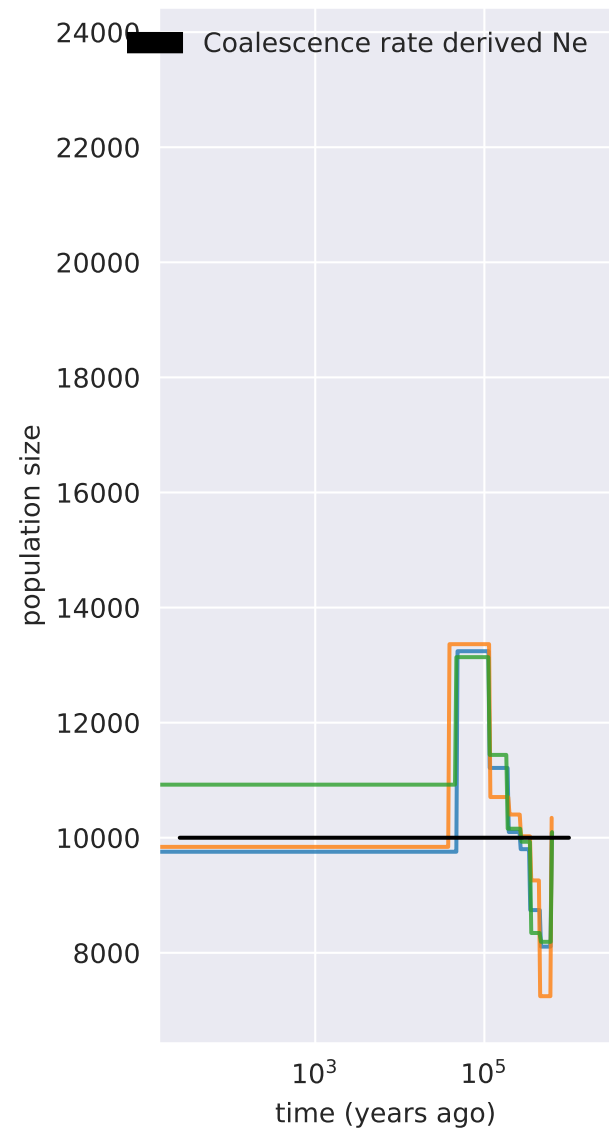
smc++
