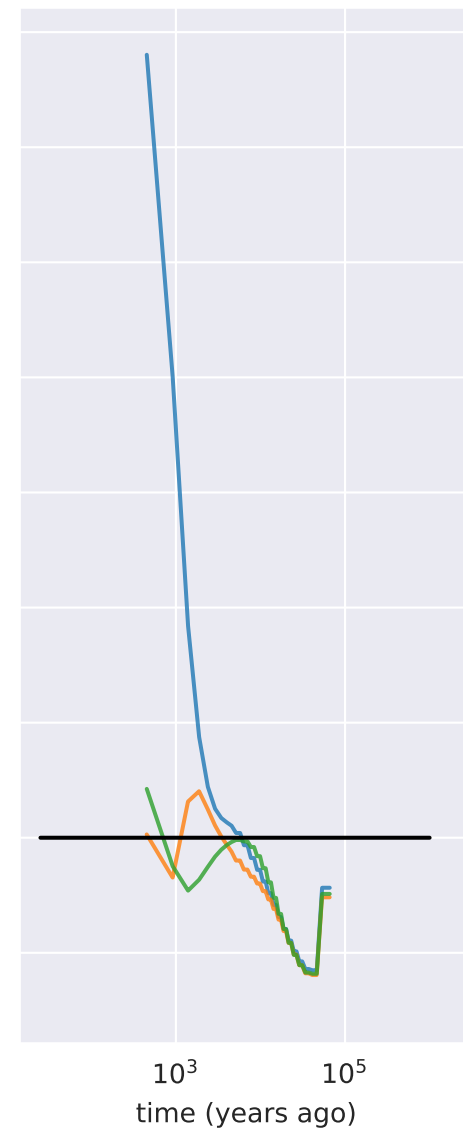
msmc, (8 samples)
