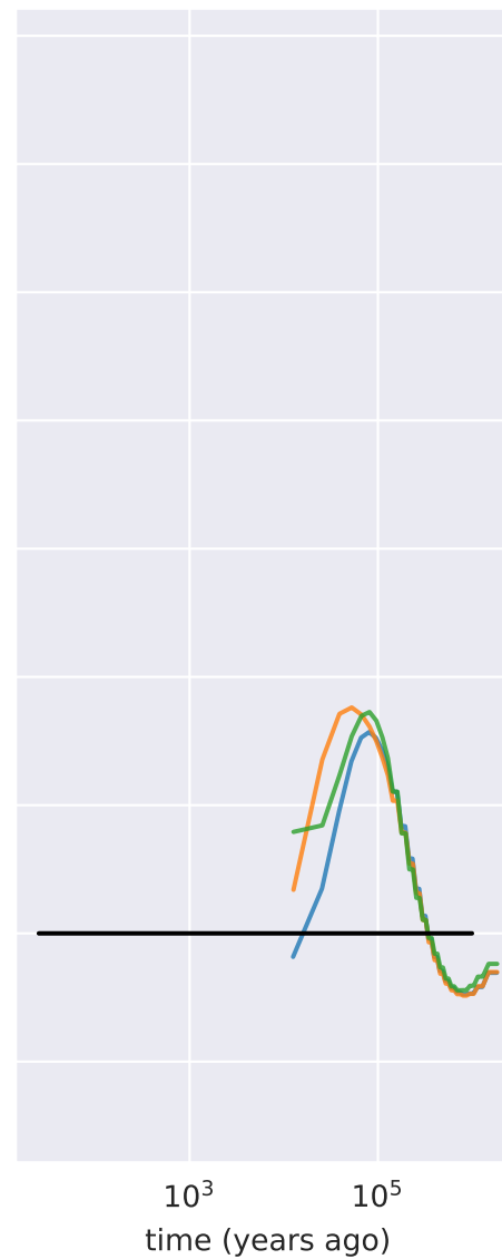
msmc, (2 samples)
